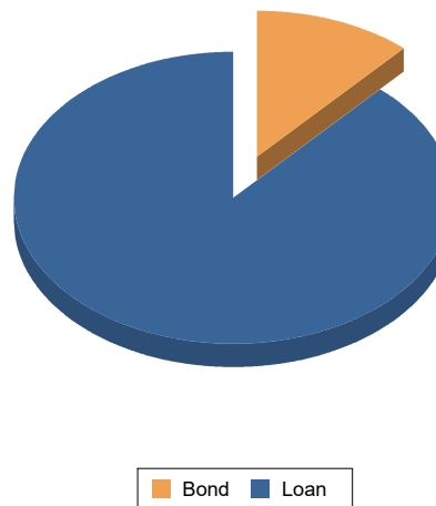
Collateral Amount by Asset Type
